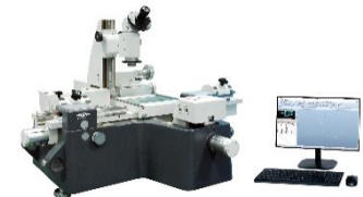
Universal Toolmaker Microscope
